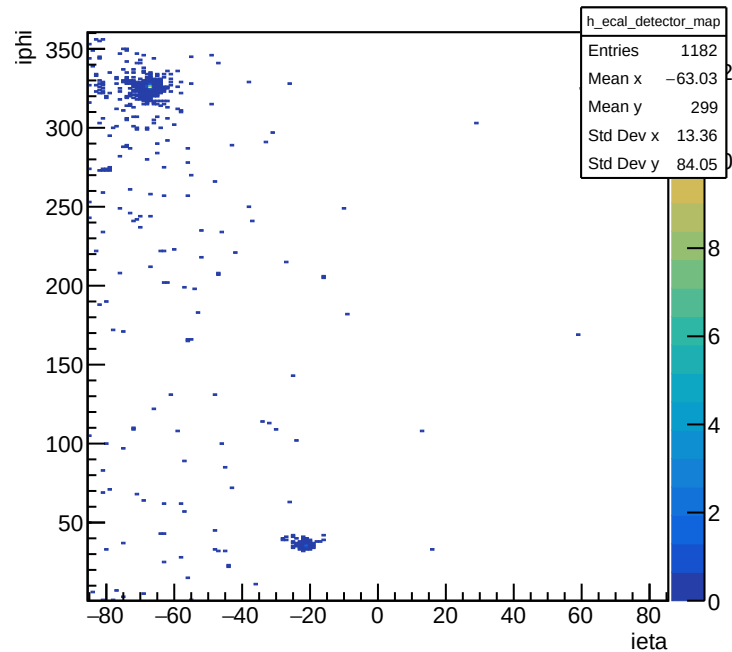
10 GeV: Resolved Photons
